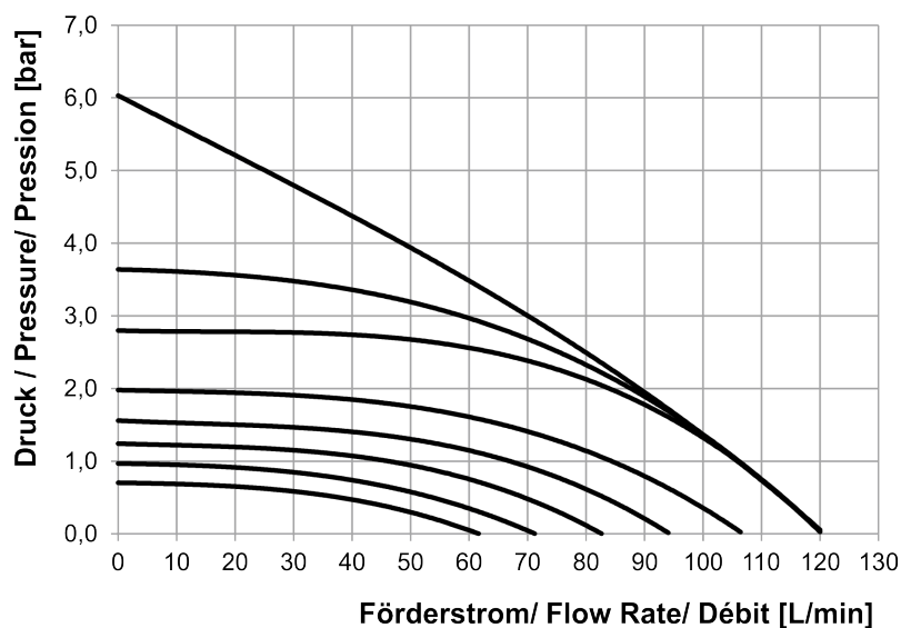
Fig. 100: Integral IN 2040 XTW, IN 2040 PW, IN 3540 XTW
